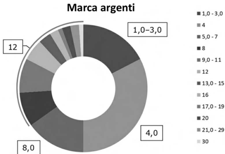
Fig. 1: The number of times a monetary value is given as a mark of silver in the RG X, in rounded percentages. N= 10,601 (circle chart).
